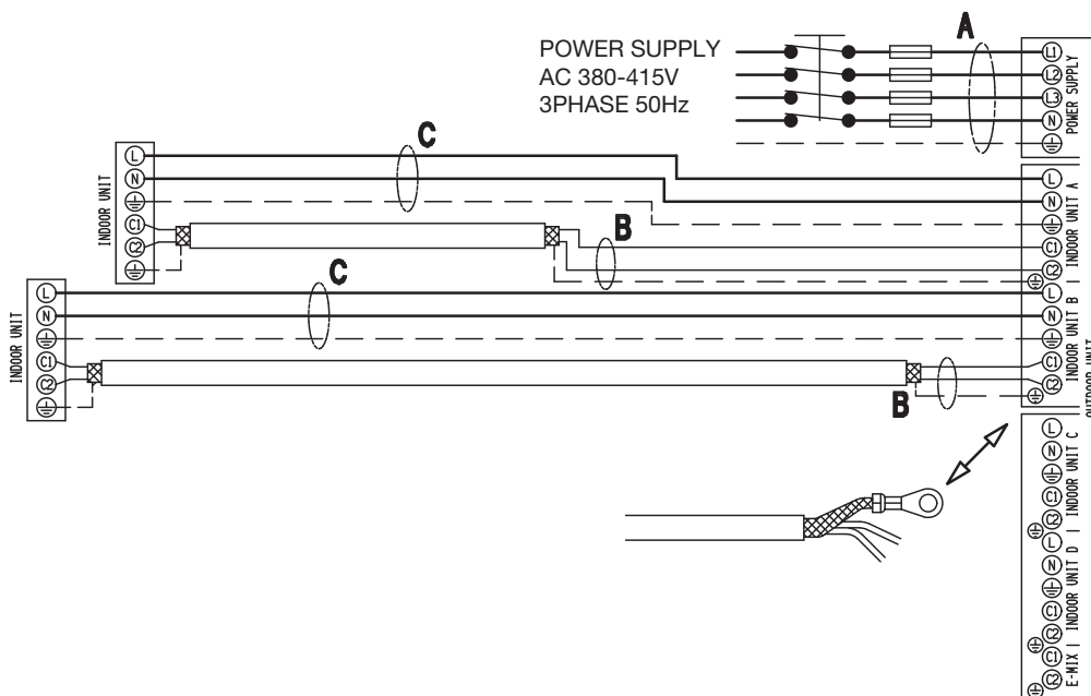
2 INDOOR UNITS 3 PHASE
